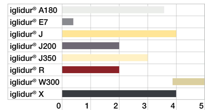
Surface pressure in thread [MPa]
