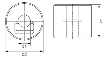
Cylindrical (form S)
