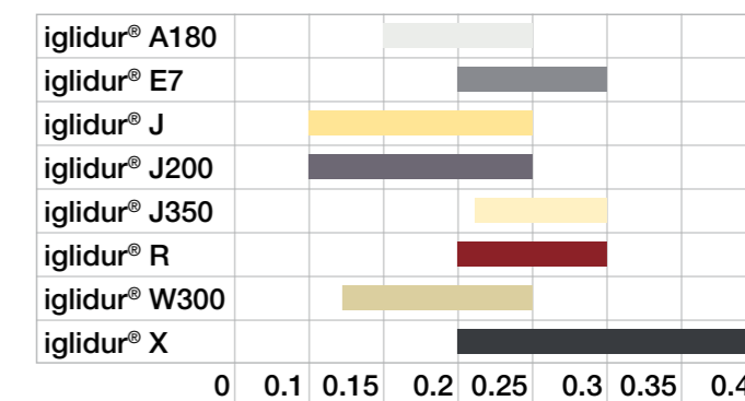
Coefficient of friction [μ]
