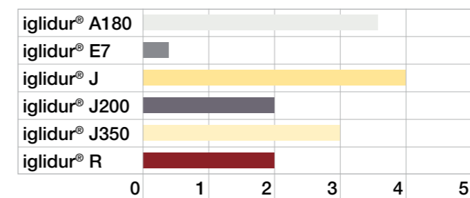
Surface pressure in thread [MPa]
