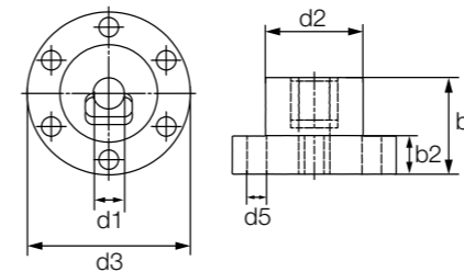
With flange (form F)
