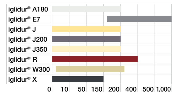
Speed [rpm]
